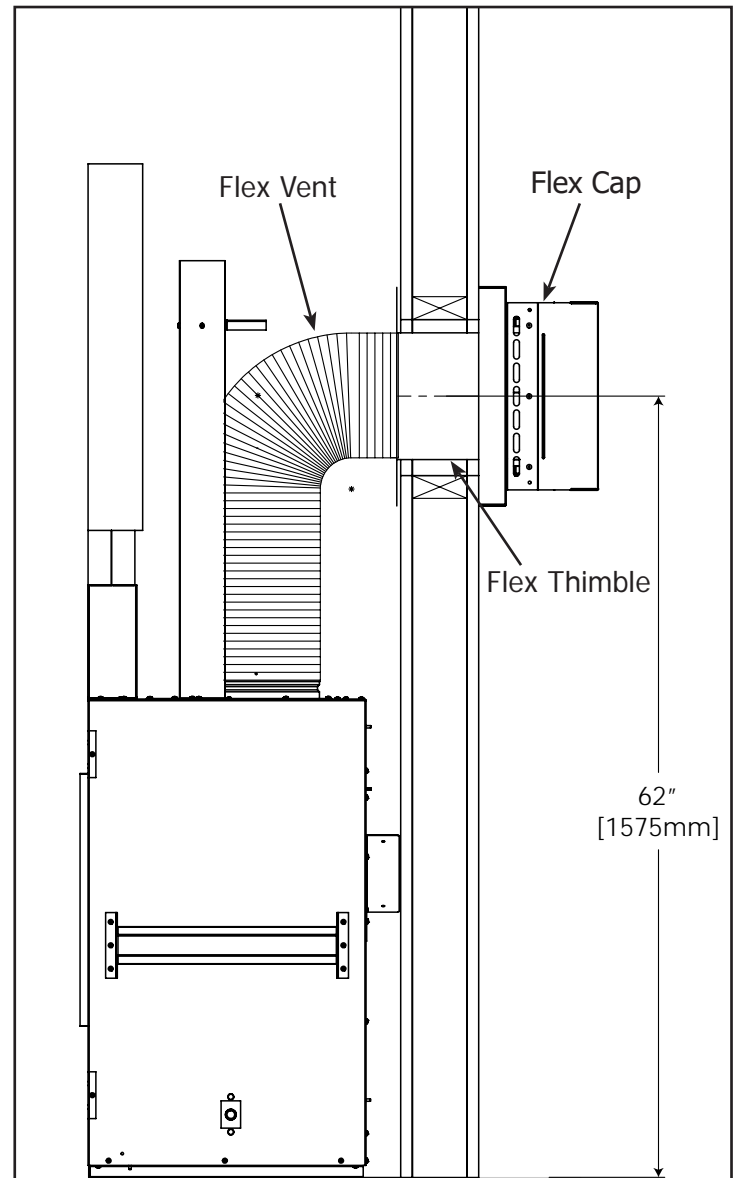
Figure 35. Flex Vent Minimum Install
