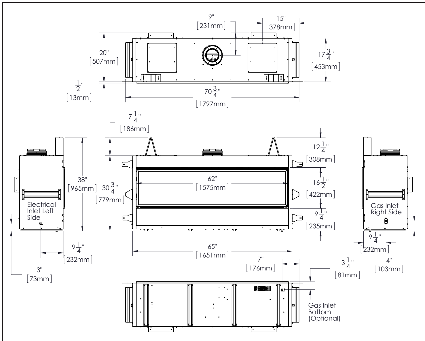
Figure 1. Unit Dimensions
