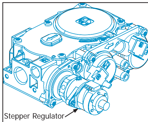
Figure 24: 885 Gas Valve
