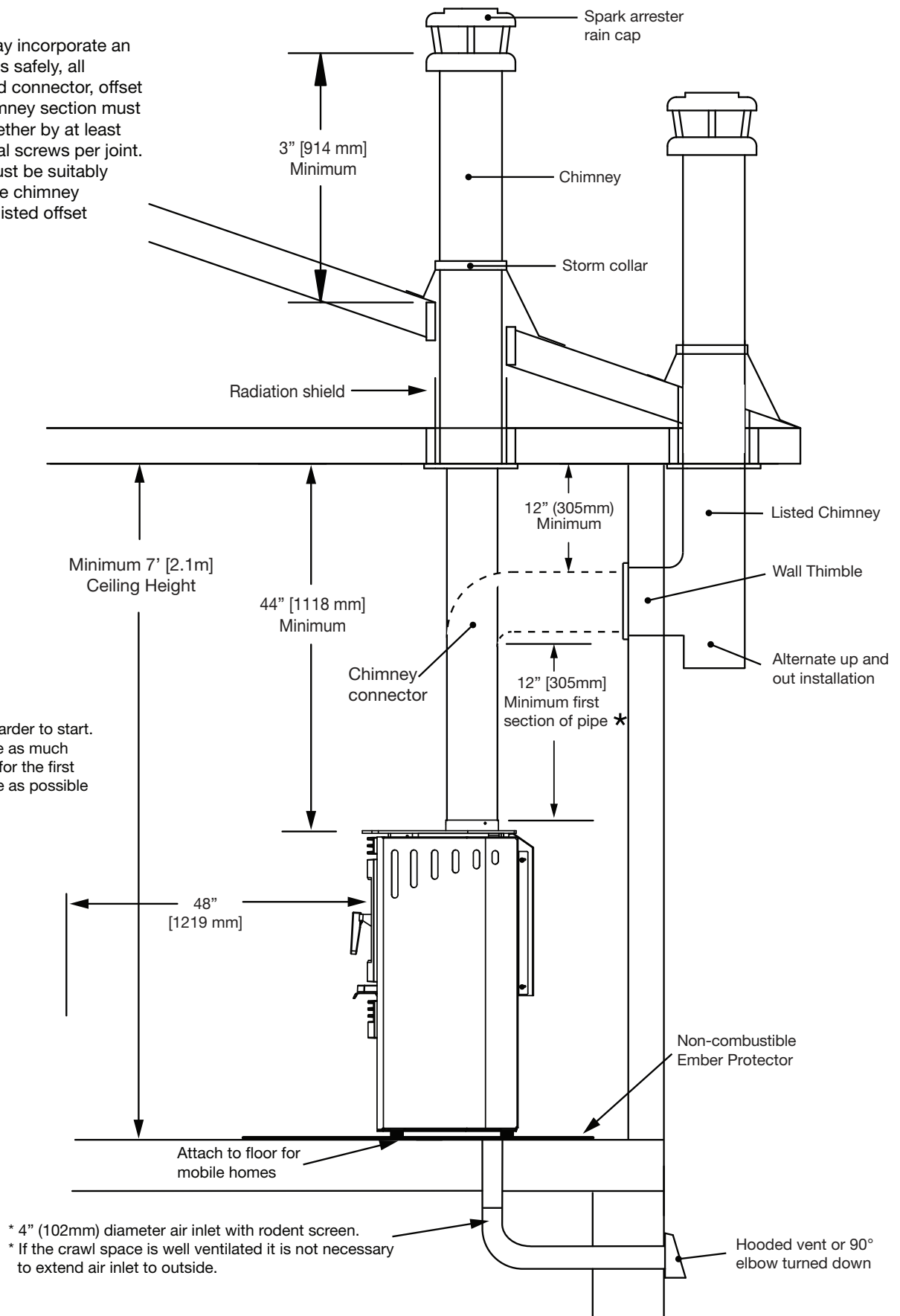
Figure 7: Residential venting.
