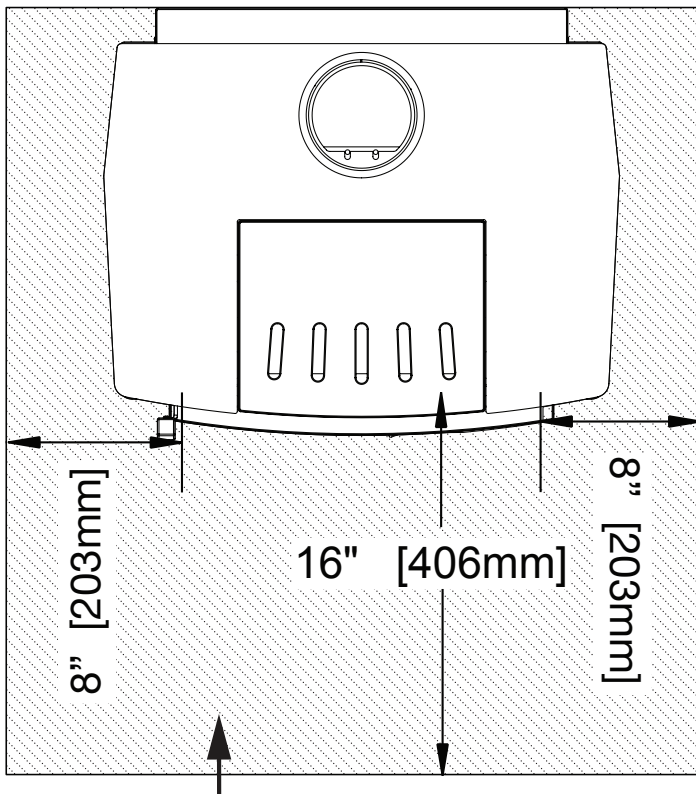
Non - combustible floor protector (Type 1 floor protector - approved to UL1618) Minimum 20GA steel
