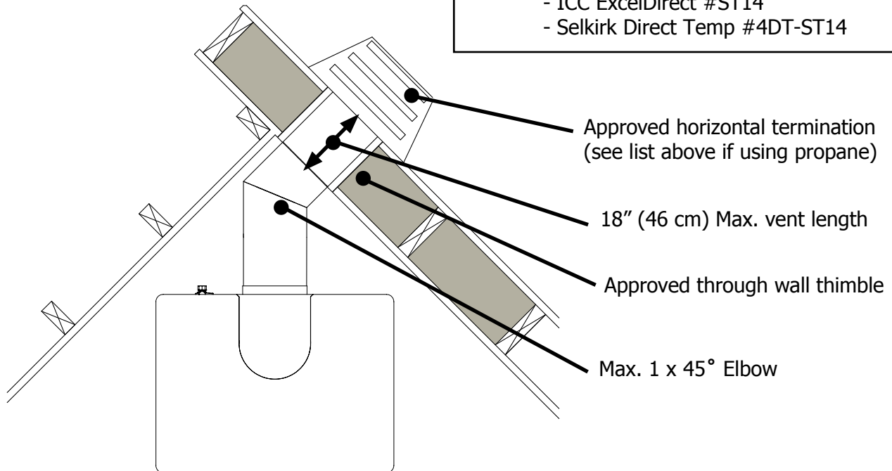
Figure 22. Corner Rear Vent - No Vertical Rise
